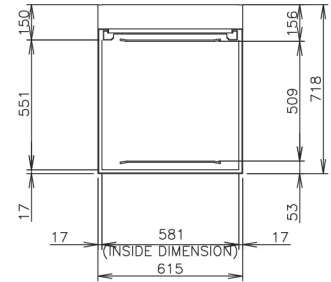
RACK SUPPORT FRAME LAYOUT STRAIGHT INSTALLATION
